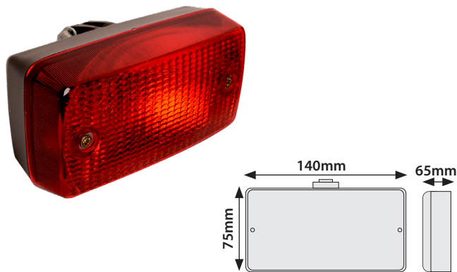
55215 Fog Lamp 12V With Mounting Bracket Bulbs Included
