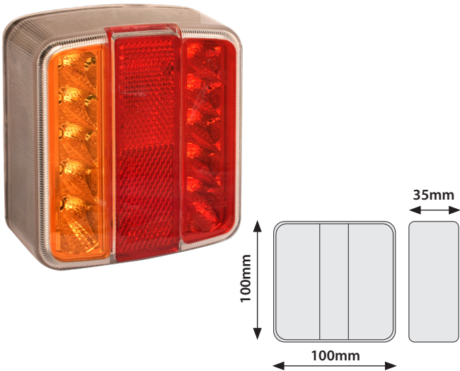
55196 LED Combination Lamp Square 12V 15cm Cable
