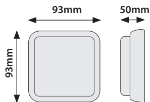
55210 LED Reverse Lamp 10-30V 40cm Cable
