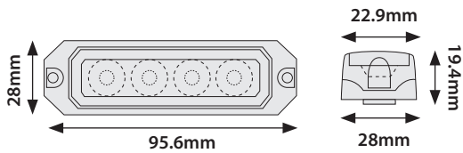
55218 LED Strobe Lamp 12W 12/24V
