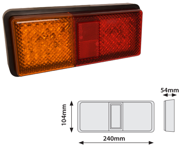
55200 Combination Lamp Rectangular EDPM Base 10-30V 40cm Cable
