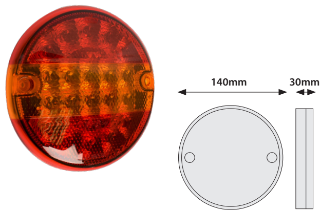
55206 LED Combination Lamp Round 9/30V Spade Connection
