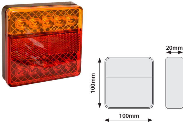
55198 LED Combination Lamp Square 12V 12.5cm Cable Slimline
