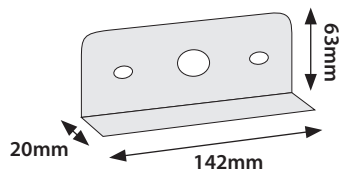
55220 Mounting Bracket 12mm Hole Diameter
