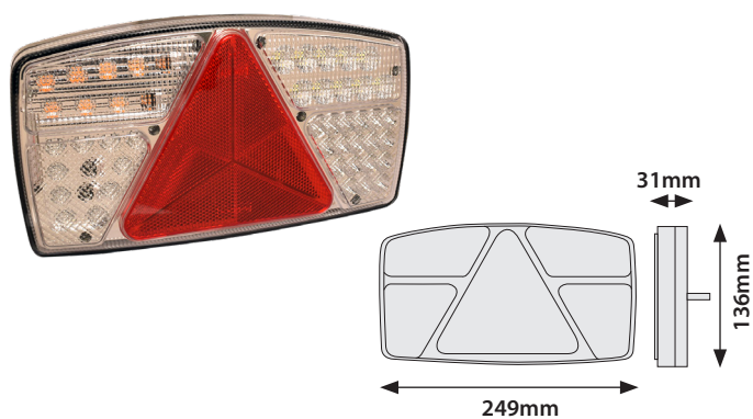
LED Combination Lamp 10/30V 54cm Cable
