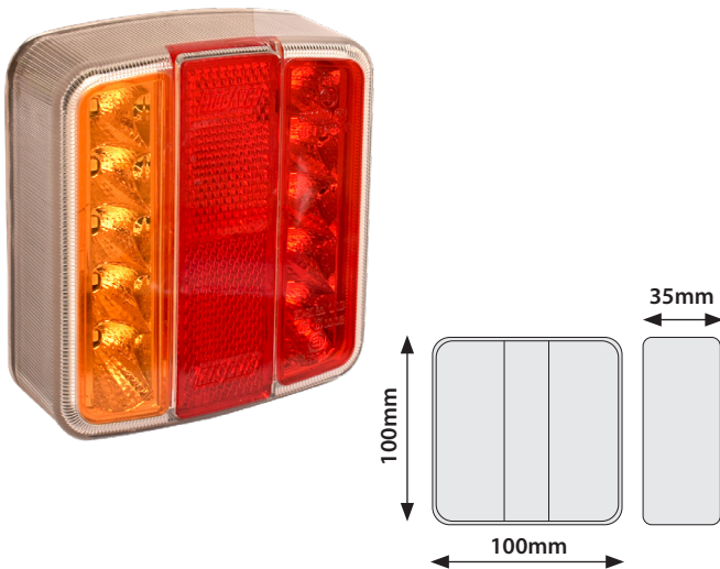
55197 LED Combination Lamp Square 12/24V 15cm Cable
