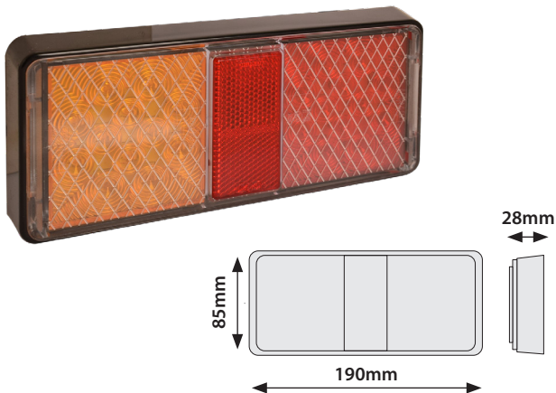
55199 LED Combination Lamp Rectangular 10/30V 30cm Cable
