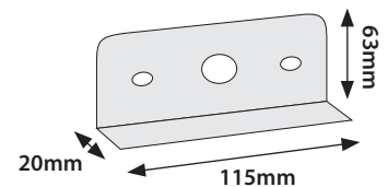
55219 Mounting Bracket For 55218 12mm Hole Diameter
