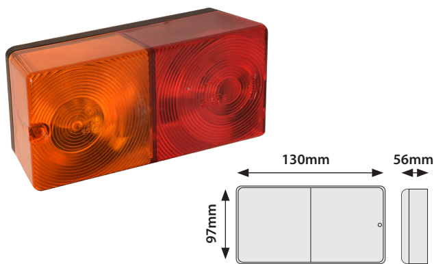
55214 Combination Lamp Rectangular 12V Bulbs Included
