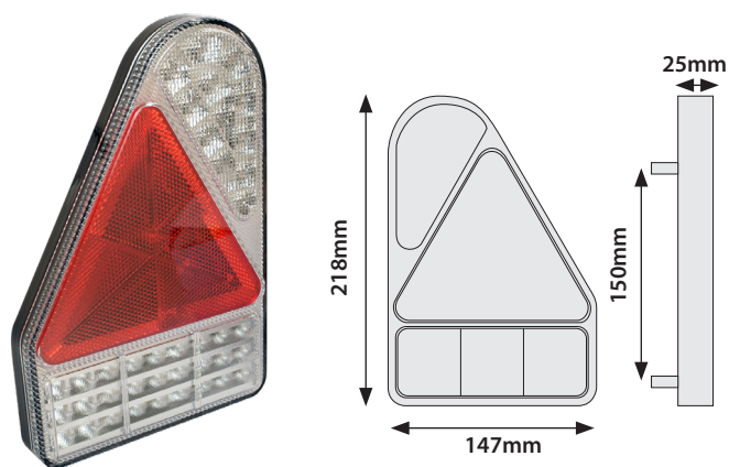
LED Combination Lamp Triangle Slimline Chrome 10/30V 45cm Cable
