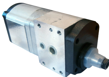
HYDRAULIC PUMP 62634R | OE Ref: 1573797116M2 Massey Ferguson 5400 5600 6200 6400 6600 7600 Series
