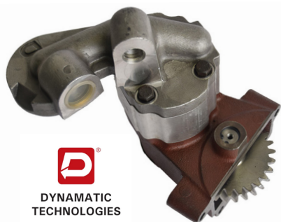
HYDRAULIC PUMP 2138 | OE Ref: 83996272 Ford 6610 7610 Eng Mounted 2000 3000s Series
