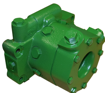
HYDRAULIC PUMP 2488 | OE Ref: AR103036 John Deere 40 50 55 Series
