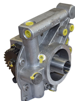
HYDRAULIC PUMP 404770R | OE Ref: 81871528 Ford New Holland 40 TS Series 3862 - Gasket 404771 | 404605 - Seal Kit
