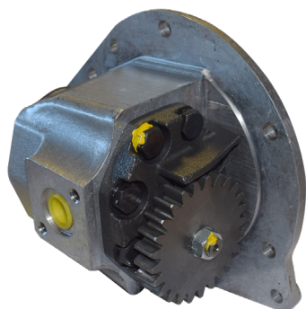
HYDRAULIC PUMP 4069R | OE Ref: 83908244 Ford 600 Series
