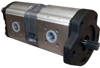
HYDRAULIC PUMP 52406 | OE Ref: 510765351 Case CS78 CS86 CS94 Bosch
