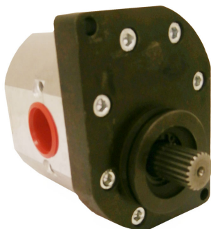
HYDRAULIC PUMP 7693 | OE Ref: 78420915 Zetor 3320/40 4320/40 5320/40 Series
