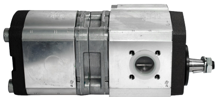
HYDRAULIC PUMP 3382280G | OE Ref: 82028450 Massey Ferguson 3000 6100 6200 3100 Series
