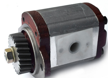
HYDRAULIC PUMP 58729 | OE Ref: RE200379 John Deere 5020 5R Series 23 cm 3 Pump Output
