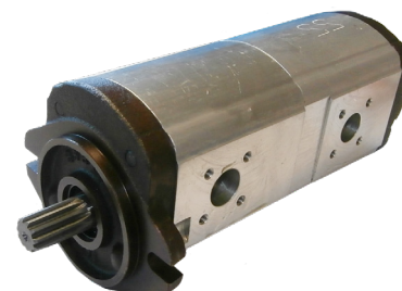
HYDRAULIC PUMP 780138 | OE Ref: 7700062603 Renault Celtis 426 436 446 456 Series
