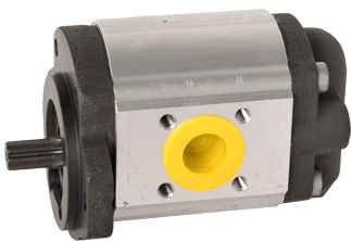
HYDRAULIC PUMP 44019 | OE Ref: 47129423 Case MXM Series Ford TM Series
