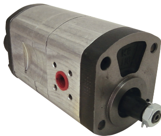
HYDRAULIC PUMP 52209R | OE Ref: 510465302 Case 33 40 43 44 45 Series
