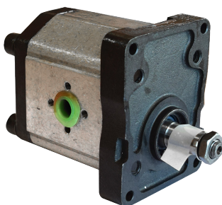
HYDRAULIC PUMP 7761 | OE Ref: 5129488 Fiat 70 - 110 90 Also fits Case JX LH Series
