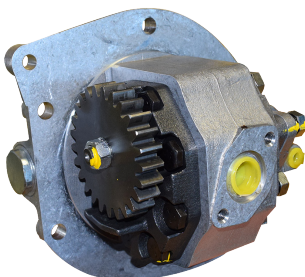
HYDRAULIC PUMP 4066R | OE Ref: 81823983 Ford 1000 Series
