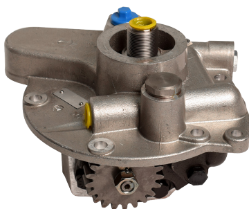
HYDRAULIC PUMP 3761R | OE Ref: 83957379 Ford 10 Series
