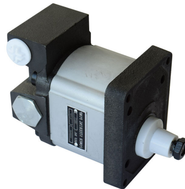
HYDRAULIC PUMP 43633R | OE Ref: 5180275 Ford 35 60 TL TM TN TLA TNA Series
