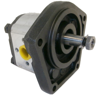
HYDRAULIC PUMP 3085 | OE Ref: 704330R95 Case 44 54 74 84 B BD Classic Series
