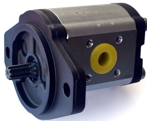
HYDRAULIC PUMP 43830 | OE Ref: 47135546 Case Maxxum MXU Series Ford T6000 TSA Series
