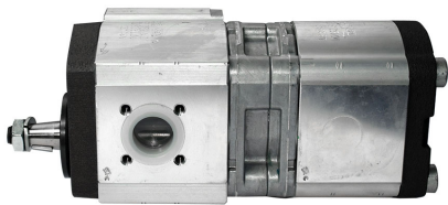
HYDRAULIC PUMP 3382280G | OE Ref: 510665389 Renault / Claas 500 Ares 500 600 Series
