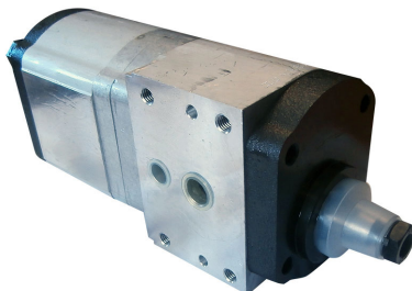
HYDRAULIC PUMP 62634R | OE Ref: 3797116M2 Renault / Claas Ares 500 600 800 Arion 600 Series
