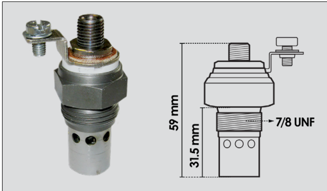
2666103 Heater Plug Old Type 12v Screw Type Large hole 20.8mm Thread OE Ref: 1854040
