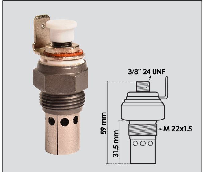
65028 Heater Plug Massey Ferguson 5400 6400 7400 Series OE Ref: 4223450M1
