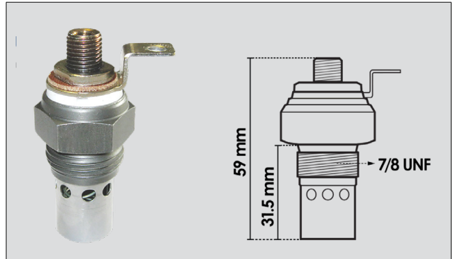
2666108 Heater Plug with Push On Connection Thread Size: 7/8" UNF OE Ref: 81806046
