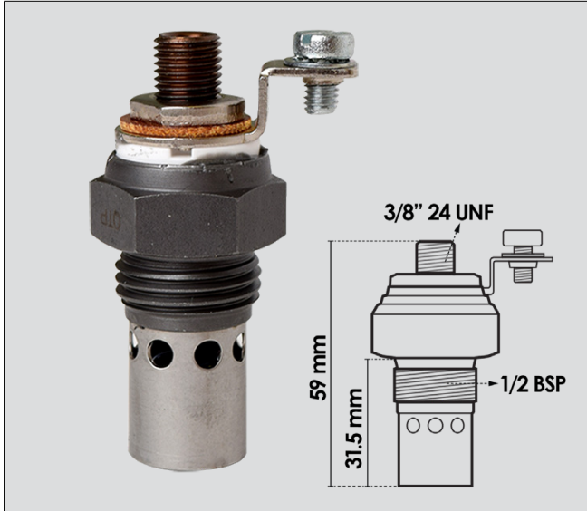
2666805 4 Cylinder Heater Plug Massey Ferguson 35 65 Series Thread Size: 1/2" BSP - 19.6mm OE Ref: 1021910M91
