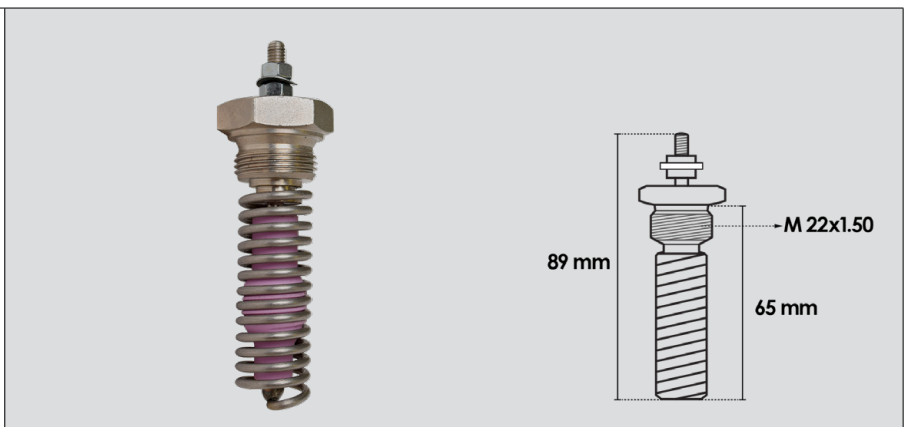
53418 Heater Plug Steyr 80 Series OE Ref: 31100090023
