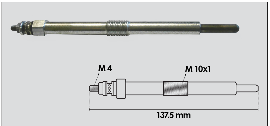
63242 Heater Plug Massey Ferguson 5425 5435 5445 5455 5460 6445 6455 6460 6470 Series OE Ref: 4224813M1
