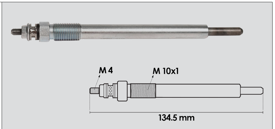
65027 Heater Plug Massey Ferguson 5445 5455 5460 5465 5475 6445 Series OE Ref: 4226560M1
