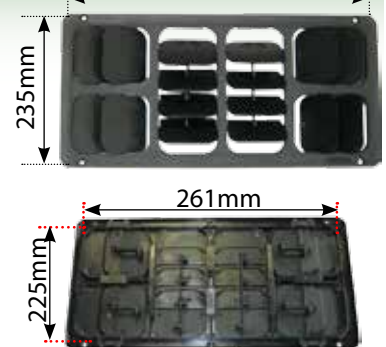
Air Vent 280 x 235mm Cut Out 261 x 225mm CX & Massey Ferguson
