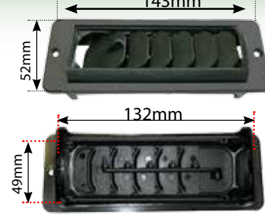
Air Vent CNH JCB 143 x 52 x 27mm Cut Out 132 x 49mm
