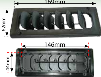
Air Vent 169 x 62 x 12mm
