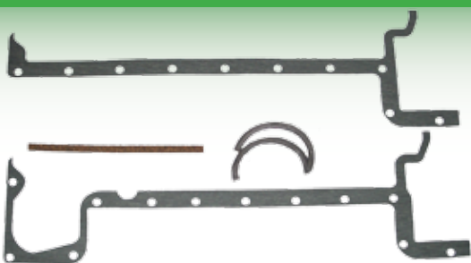
1096 Sump Gasket Set Major Super Major
