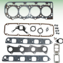
Q2830920 Gasket Cylinder Head 1.15mm 4 Cylinder NEF OE Ref: 2830920
